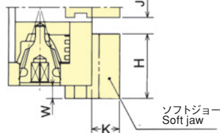
(SC-14, 16の取付60°ピッチ=6本) (Mounting of SC-14, 16: 60° pitch 6 pcs.)
