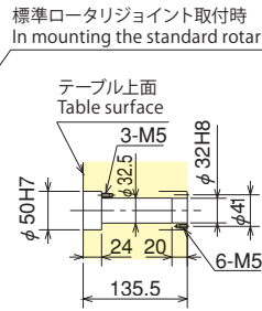
テーブル貫通穴 Through Hole Diameter
