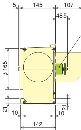
テーブル貫通穴 Through Hole Diameter
