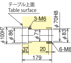
テーブル貫通穴 Through Hole Diameter
