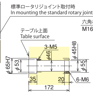
テーブル貫通穴 Through Hole Diameter
